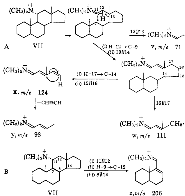
Scheme I. Primary 9–11 Cleavage (A) and 10–11 Cleavage (B)
