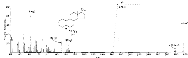
Figure 2. Mass spectrum of 6β-dimethylaminocholestane (V).
