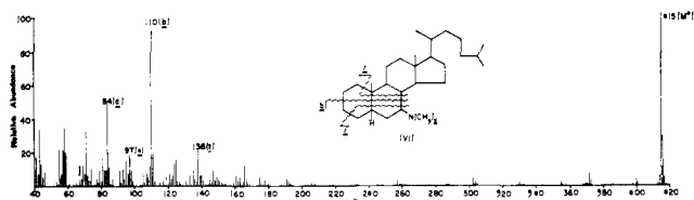
Figure 3. Mass spectrum of 7 \beta -dimethylaminocholestane (VI).
