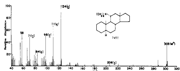
Figure 4. Mass spectrum of 11 \alpha -dimethylamino-5 \alpha -androstane (VII).
