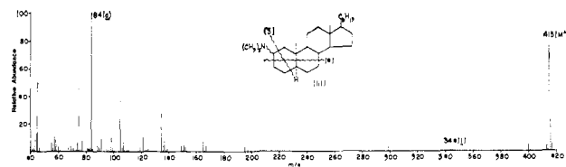
Figure 1. Mass spectrum of 2-dimethylaminocholestane (III).
