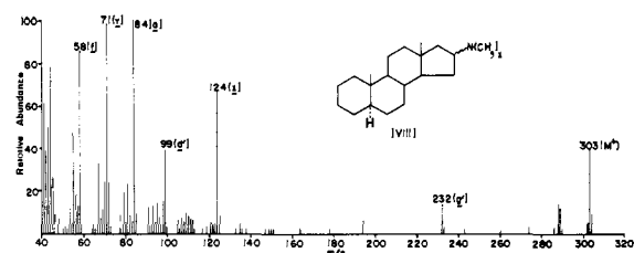
Figure 5. Mass spectrum of 16 \xi -dimethylamino-5 \alpha -androstane (VIII).
